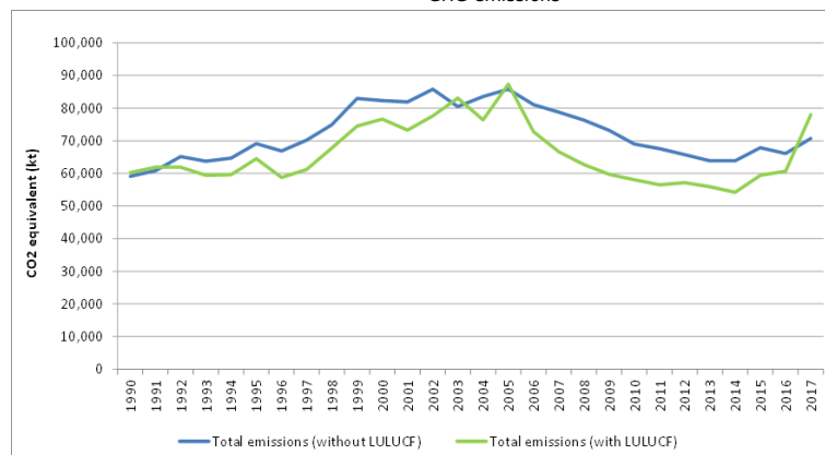
Figure III.4 GHG emissions
